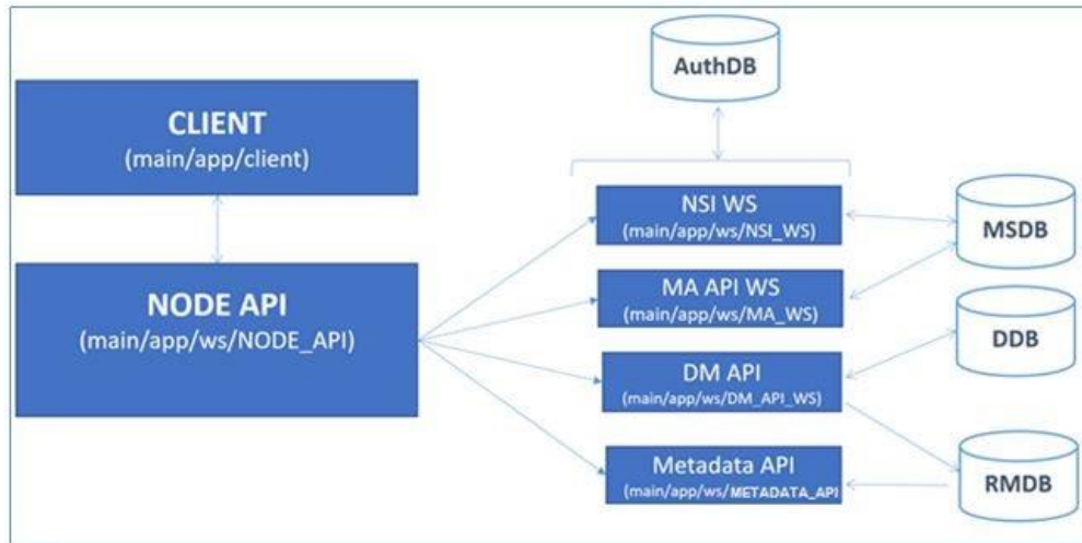
Software architecture
